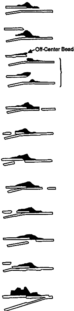
FIG. 4 Locus-of-Break Codes for Fillet Extrusion Weld Seams in Unreinforced Geomembranes Tested for Seam Strength in Shear and Peel Modes
