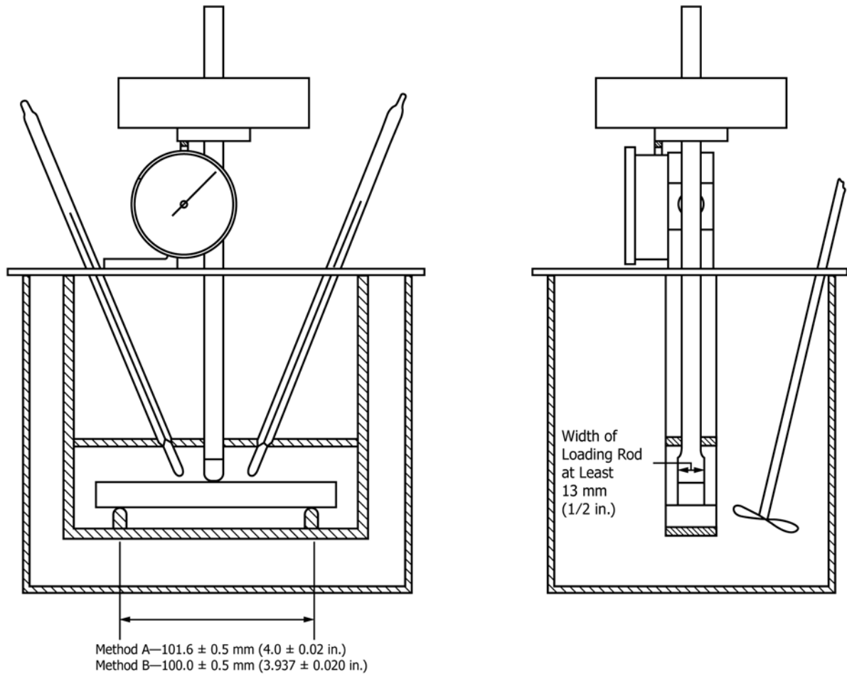
FIG. 1 Apparatus for Deflection Temperature Test
